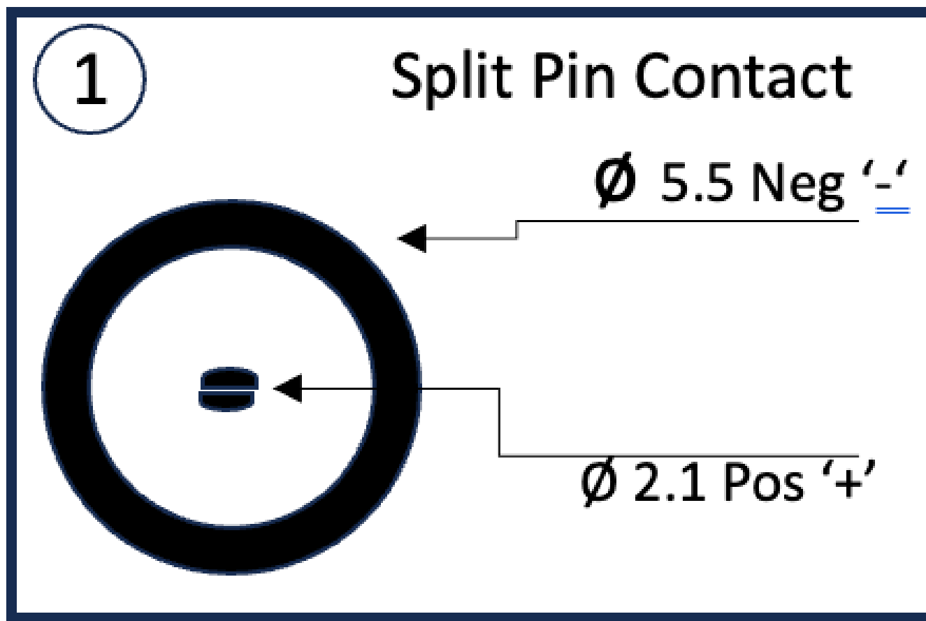
Connector A
