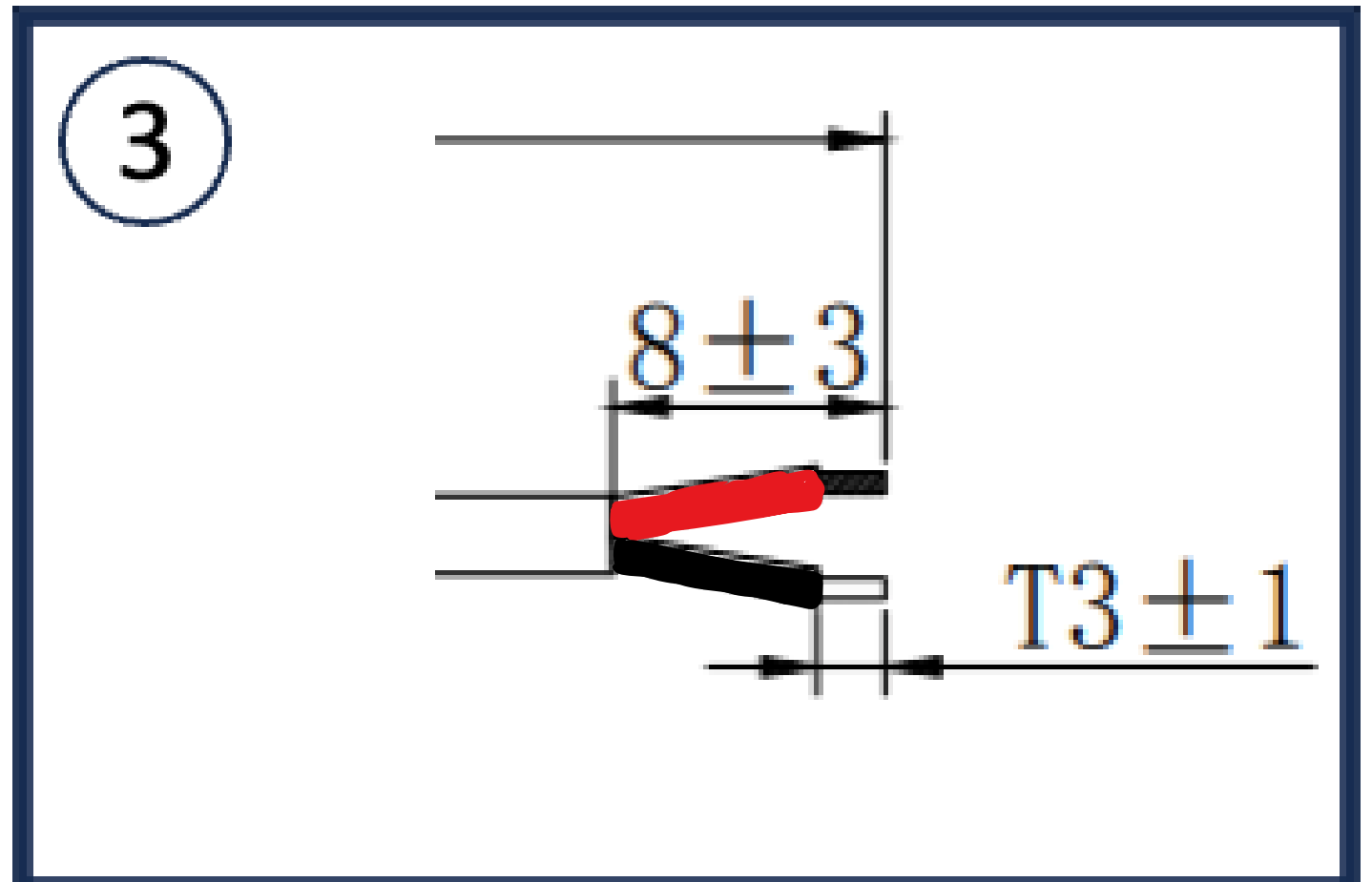
Connector B
