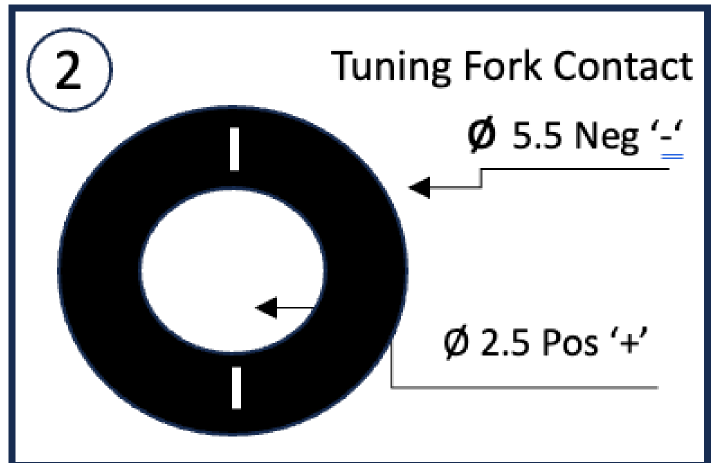
Connector B
