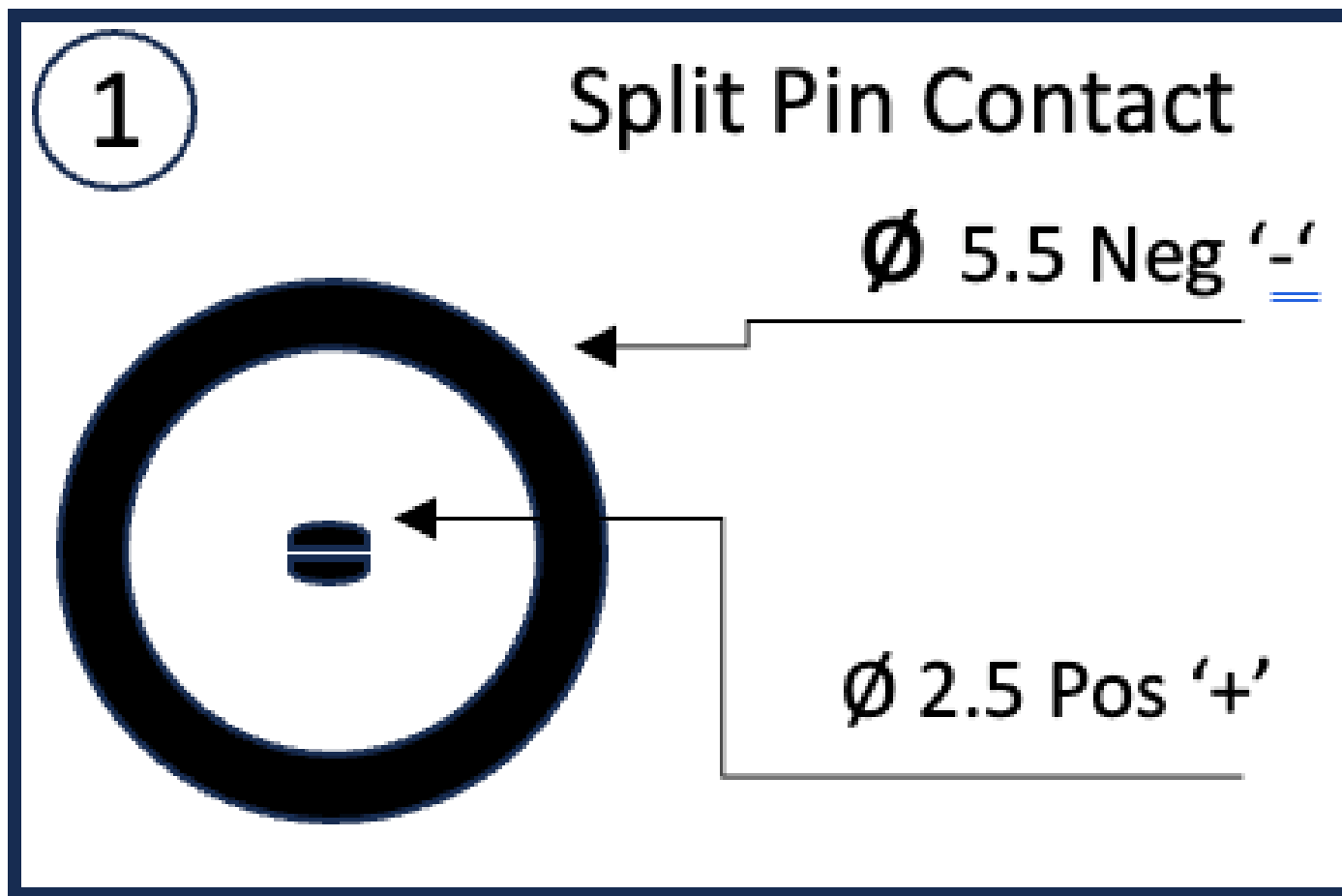
Connector A
